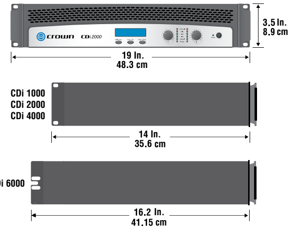
Figure 2.1 Dimensions
